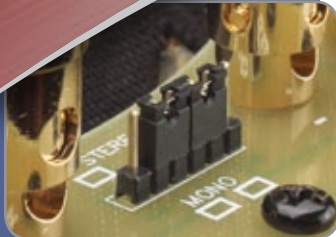
Jumpers setting for either Conventional/Surround or Single-Point Stereo Use
